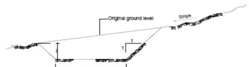
CROSS-SECTION C-C (PROTECTIVE TRENCH) Scale 1:100
