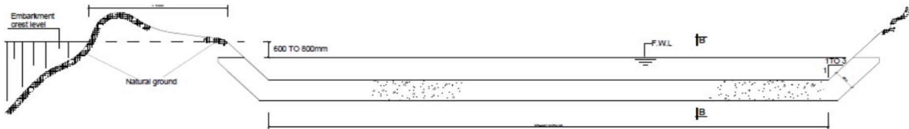
CROSS-SECTION A-A (SPILLWAY CREST)
