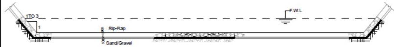
SPILLWAY PROTECTION ARRANGEMENT Scale 1:100
